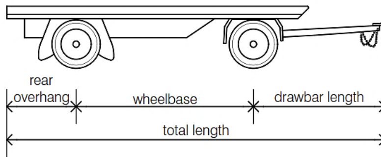
Key length dimensions of dog trailers
