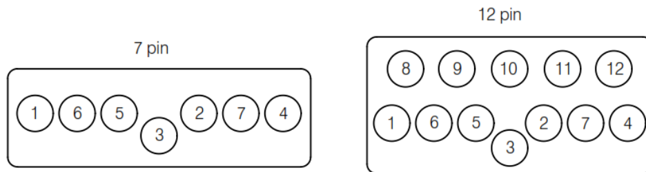
Front view of 7-pin and 12-pin trailer plugs
