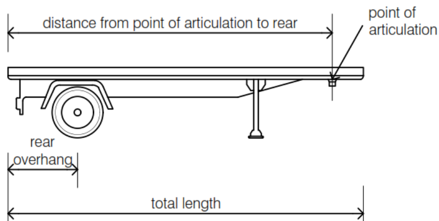
Key length dimensions of semi-trailers
